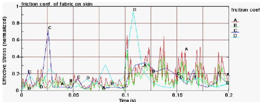
Fig. 3 Normalized effective stresses at different friction coefficients as a function of time for simulation b: (A) 0.3, (B) 0, (C) 0.2, and (D) 0.5
